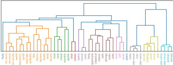
Figure 1: Hierarchical clustering dendrogram of the MagnaTagATune music tags.
